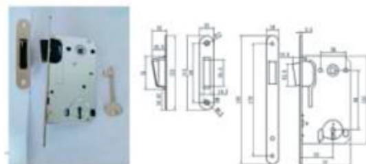
9050-KEY HOLE UPPER LATCH
