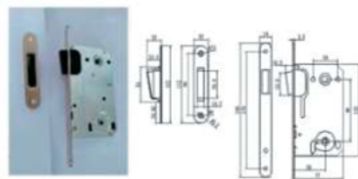
9050-WC UPPER LATCH
